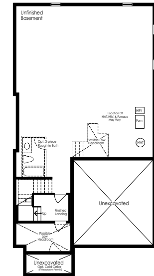
Basement for Opt. Loft Elevation A & B
