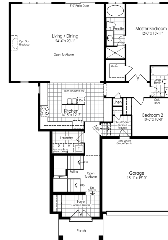
Ground Floor For Opt. Loft Elevation A
