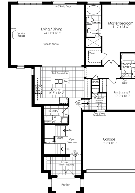
Ground Floor For Opt. Loft Elevation B
