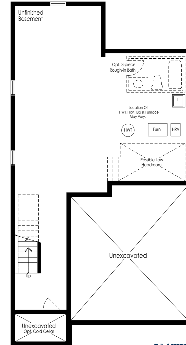
Basement Elevation A, B & C
